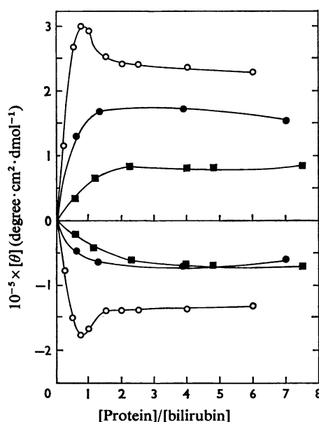
Fig. 5. Ellipticity of bound bilirubin as a function of albumin or fragment concentration
